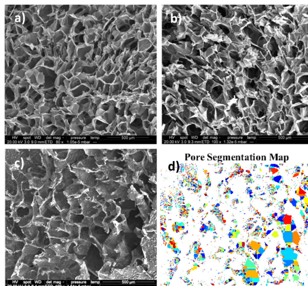
Fig. 6 SEM captured images of 3 (wt)% chitosan scaffold; a). 0 mg ml -1 doxycycline loaded, b). 10 mg ml -1 doxycycline loaded, c). 40 mg ml -1 doxycycline loaded; d) indicative segmentation map for determining porosity for 40 mg ml -1 DOX sample.
