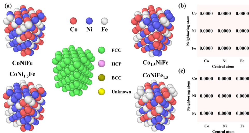
Fig. 1 (a) The primitive unit cell of the equiatomc MEA (CoNiFe) and three non-equiatomc MEAs (Co 1.5 NiFe, CoNi 1.5 Fe, and CoNiFe 1.5 ) and their phase structure. (b) The WCP of equiatomc MEA. (c) The WCP of three non-equiatomc MEAs.
