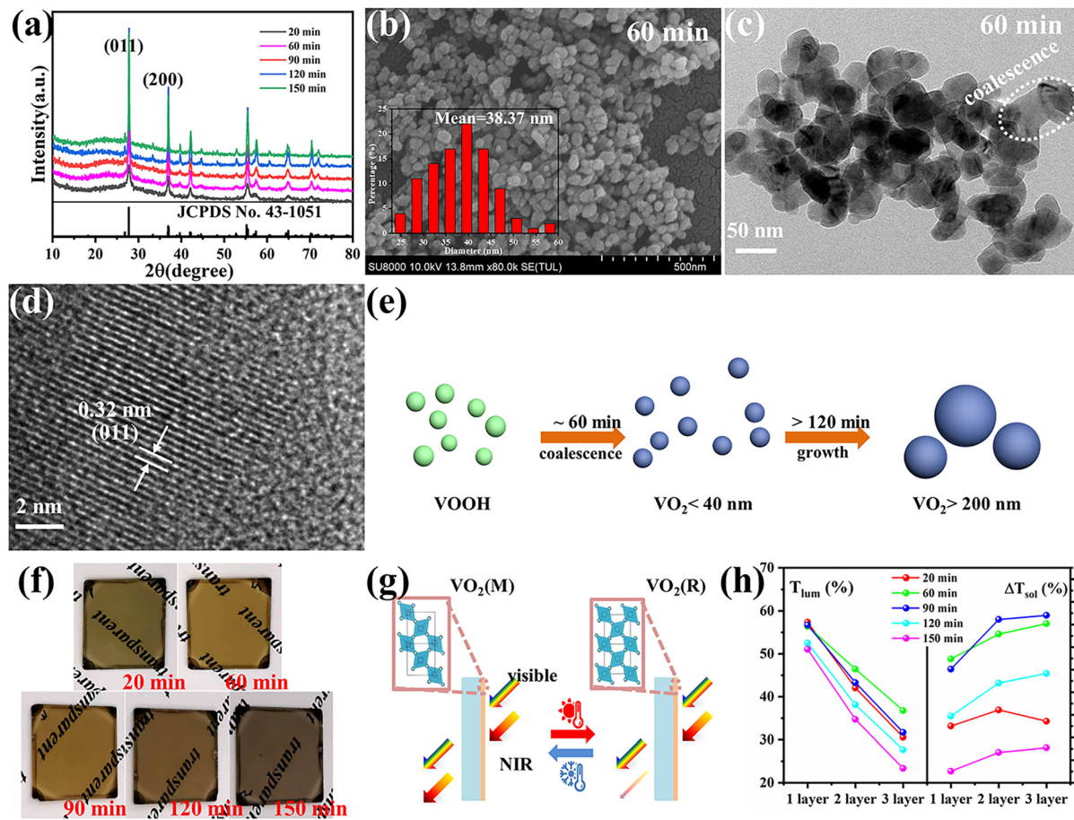
Fig. 3 (a) XRD patterns of \text{VO}_2 with different annealing times. (b) SEM and (c) and (d) TEM images of \text{VO}_2 with annealing a time of 60 min. (e) Schematic illustrations of the transformation of VOOH into \text{VO}_2 . (f) Digital images of \text{VO}_2/\text{PVP} films. (g) Working principle of the \text{VO}_2 -based smart window. (h) The optical performances of \text{VO}_2/\text{PVP} films with various spin coating times. (Inset (b): histogram of size distribution of the \text{VO}_2 NPs).
