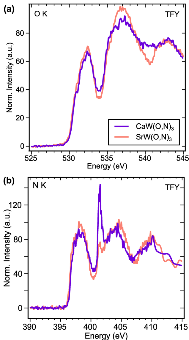
Fig. 5 (a) Oxygen and (b) nitrogen K-edge XAS spectra of \text{CaW}(\text{O,N})_3 and \text{SrW}(\text{O,N})_3 perovskite powder samples measured in total fluorescence yield. Intensities are area-normalized between 528–545 eV for O K-edge and 394–410 eV for N K-edge.
