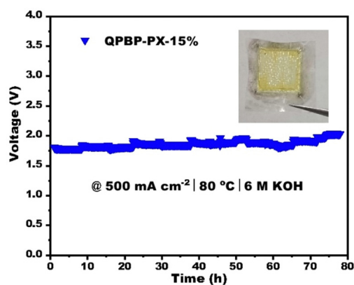
Fig. 7 Durability of QPBP-PX-15% based AEMWE at 80 °C, 500 mA cm -2 , and in 6 M KOH solution.
