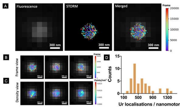
Fig. 2 STORM characterization of urease molecules around the nanomotors. (A) STORM recorded localisations of Cy5-labelled enzymes are superimposed on the FITC fluorescence image for better visualization. The colour of a localisation represents the frame in which it was recorded. Scale bars are 300 nm. (B) Representative STORM images showing urease localizations in a nanomotor. (C) Corresponding images showing the localization density, where the distribution of urease can be visualized. (D) Histogram of the number of urease localisations per analysed nanomotor. The results are shown as the mean \pm SD ( N = 41 ).
