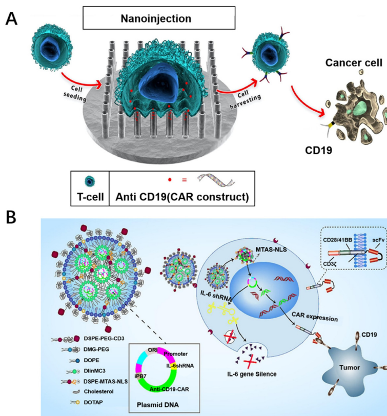
Fig. 3 Biomaterial designs for promoting the transfection of CAR-T cells. (A) Vertically aligned silicon nanotube arrays successfully transfect CAR into primary T cells. Reproduced with permission. 62 Copyright 2023, Elsevier. (B) A lipid nanoparticle system with a surface modified with CD3 antibodies was constructed containing plasmids of interleukin 6 short hairpin RNA (IL-6 shRNA) and CD19-CAR (antiCD3-LNP/CAR19 + shIL6) combination genes to stably transfect T cells. Reproduced with permission. 66 Copyright 2022, Elsevier.
