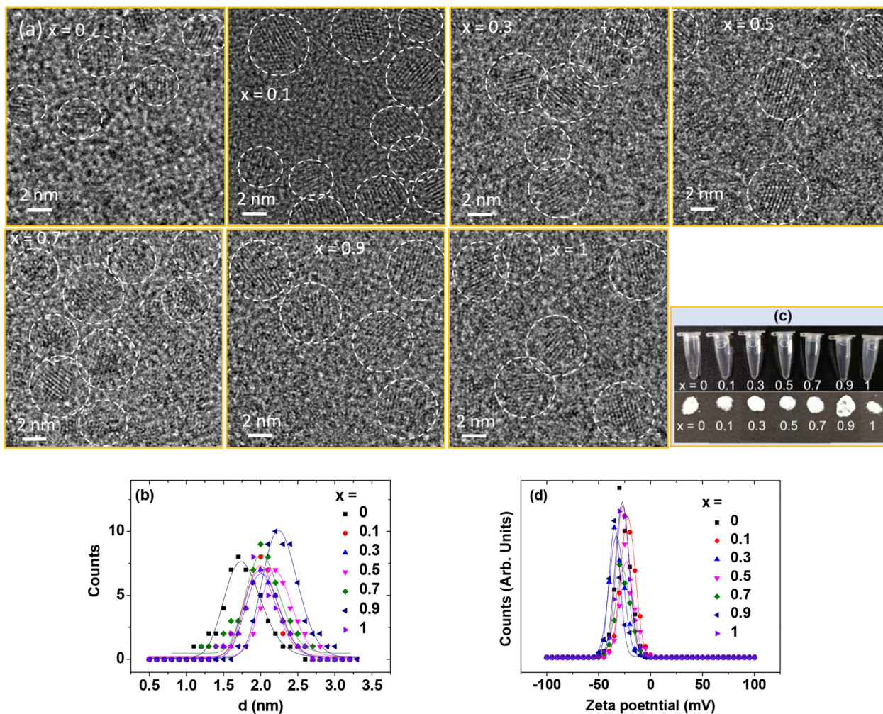
Fig. 2 \text{GdEu}_x\text{Tb}_{1-x}\text{O}_3@/\text{PAA}/\text{PDA} nanoparticles ( x = 0, 0.1, 0.3, 0.5, 0.7, 0.9, and 1 ): (a) HRTEM images, (b) log-normal function fits depicting the observed particle diameter distributions, (c) images of solution samples (top), showing good colloidal stability in aqueous media, and powder samples (bottom), and (d) zeta potential curves and Gaussian function fits.
