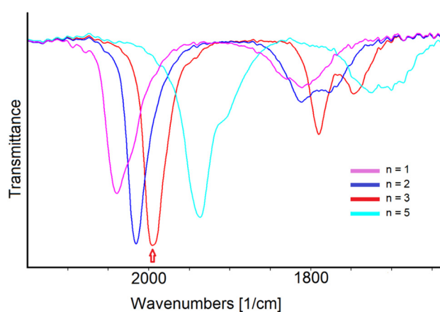
Fig. 6 Selected infrared spectra of [\text{Rh}_{12}\text{In}(\text{CO})_{28}]^{n-} as a function of the cluster charge n in \text{CH}_3\text{CN} containing 0.1 \text{ mol dm}^{-3} [\text{N}^{\text{t}}\text{Bu}_4][\text{PF}_6] . The absorptions of the solvent and supporting electrolyte have been subtracted. The red arrow indicates the initial spectrum.
