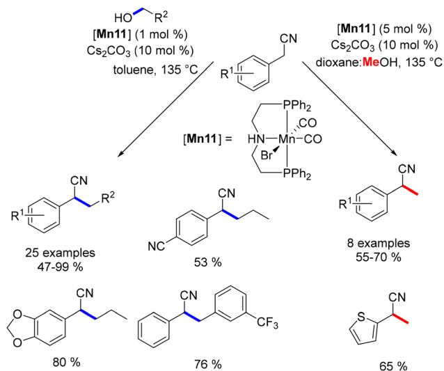
Scheme 58 Alkylation of nitriles, as reported by Rueping.
