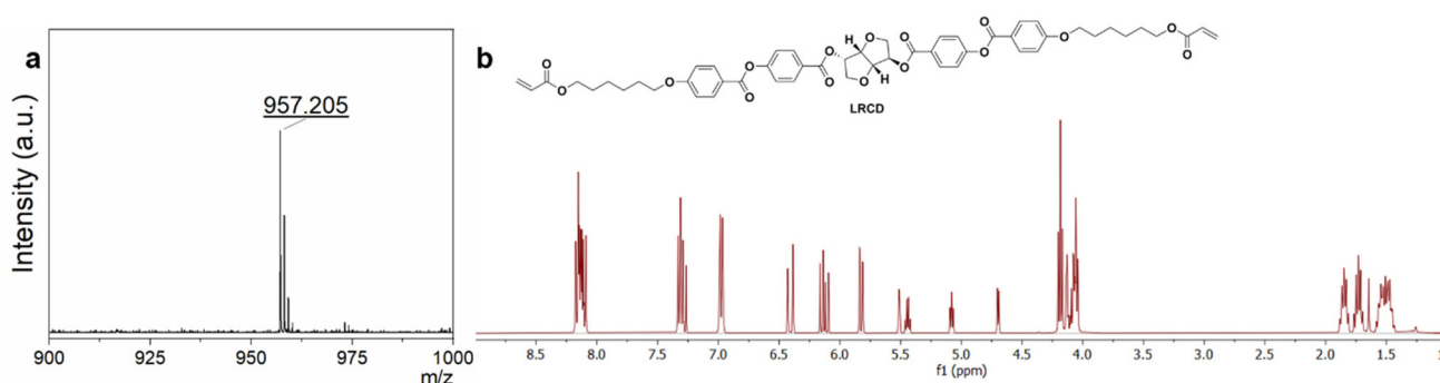
Fig. 1 (a) MALDI-TOF-MS measurement of LRCD . (b) The ^1\text{H-NMR} spectrum of LRCD in \text{CDCl}_3 .
