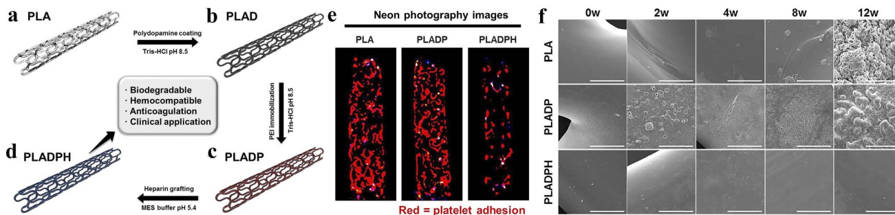
Fig. 8 (a) 3D printed bare PLA stent. (b) PDA coating on bare PLA stent. (c) PEI immobilization on PDA coated PLA stent. (d) Hep grafting on PDA/PEI layered PLA stent. (e) Neon photography images for platelet visualization on PLA, PLADP, and PLADPH ( n = 3 ). (f) Surface morphology variation of the PLA, PLADP, and PLADPH throughout the specific time points degraded in PBS solution under pH 7.4 at 37 °C. Reproduced from ref. 97 with permission from Elsevier, copyright 2019.
