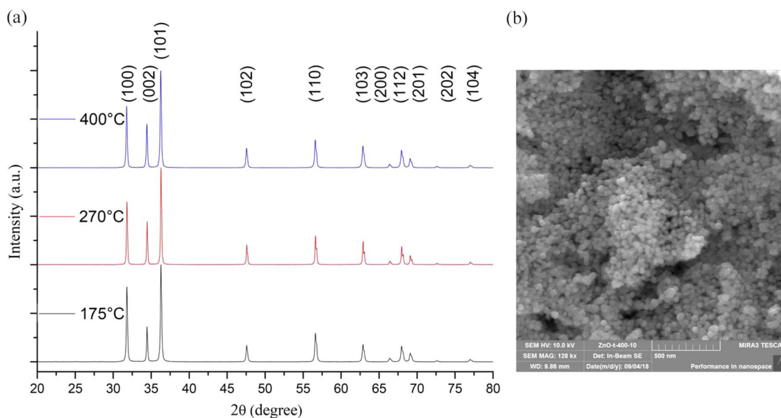
Fig. 4 XRD patterns of ZnO samples annealed at different temperatures (a) and an electron microscopic image of a ZnO sample subjected to thermal treatment at a temperature of 400 °C (b). 31
