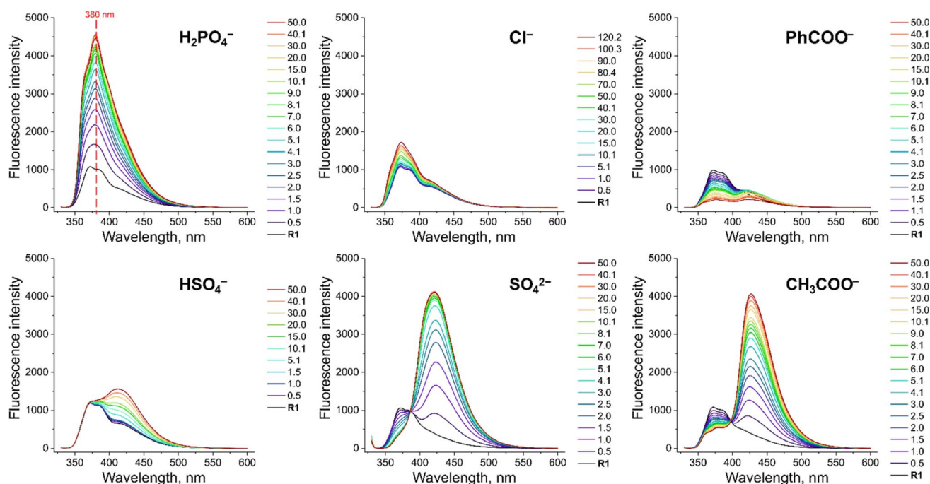
Fig. 3 Fluorescence spectra of 10 \mu\text{M} R1 in the presence of various TBA salts in DMSO/0.5% H 2 O at 298 K. EX WL: 324 nm.
