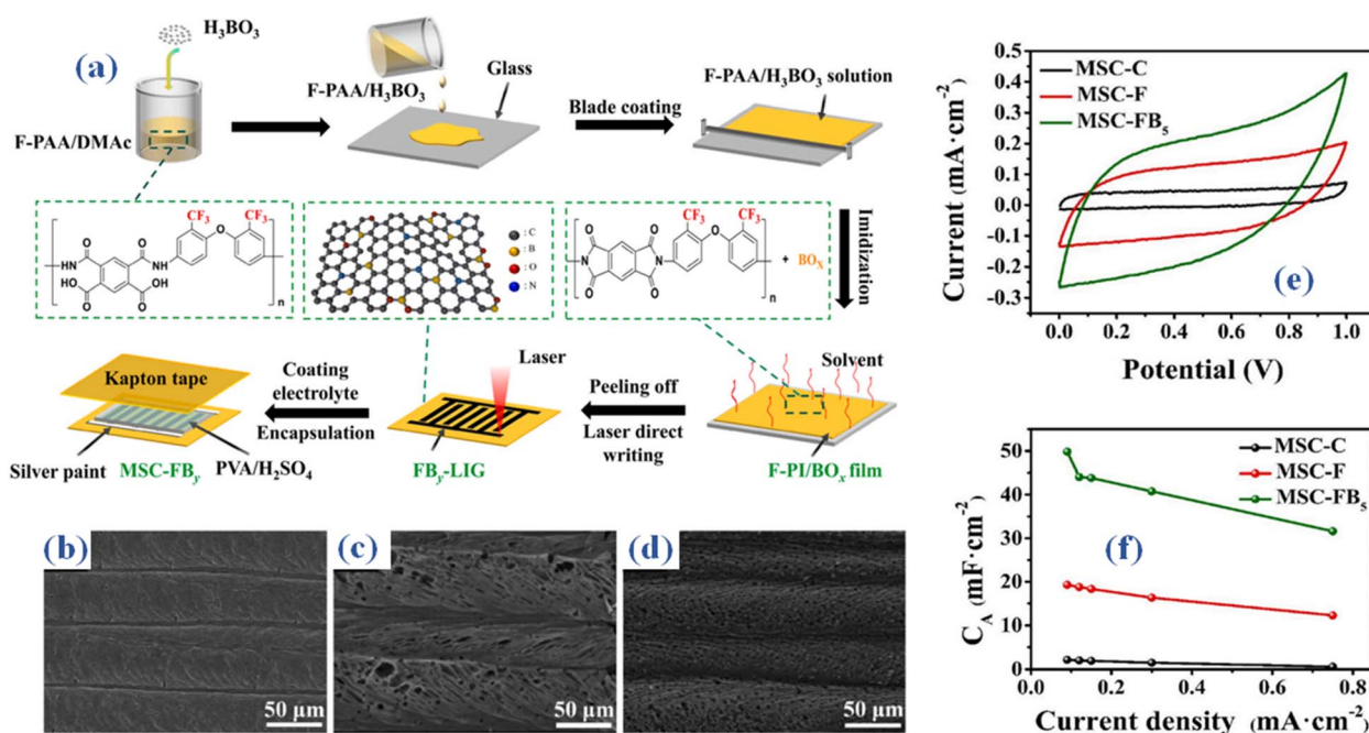
Fig. 3 (a) Schematic representation of F-PI/ \text{Bo}_x film fabrication process (b-d) SEM outcomes of fabricated films (e) the CV curves for MSC-C, MSC-F, and MSC-FB 5 (f) areal capacitance at different current densities. 32
