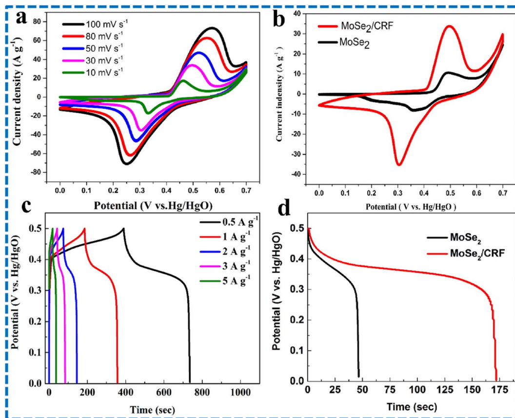
Fig. 18 (a) CV plot of the MoSe 2 /CRF composite at different scan speeds, (b) CV plot of MoSe 2 and the composite at 30 mV s -1 , (c) GCD curves of the composite at different current densities, (d) discharging profiles for MoSe 2 and the composite electrode at 1 A g -1 . This figure has been reproduced from ref. 105 with permission from Elsevier, Copyright 2021.
