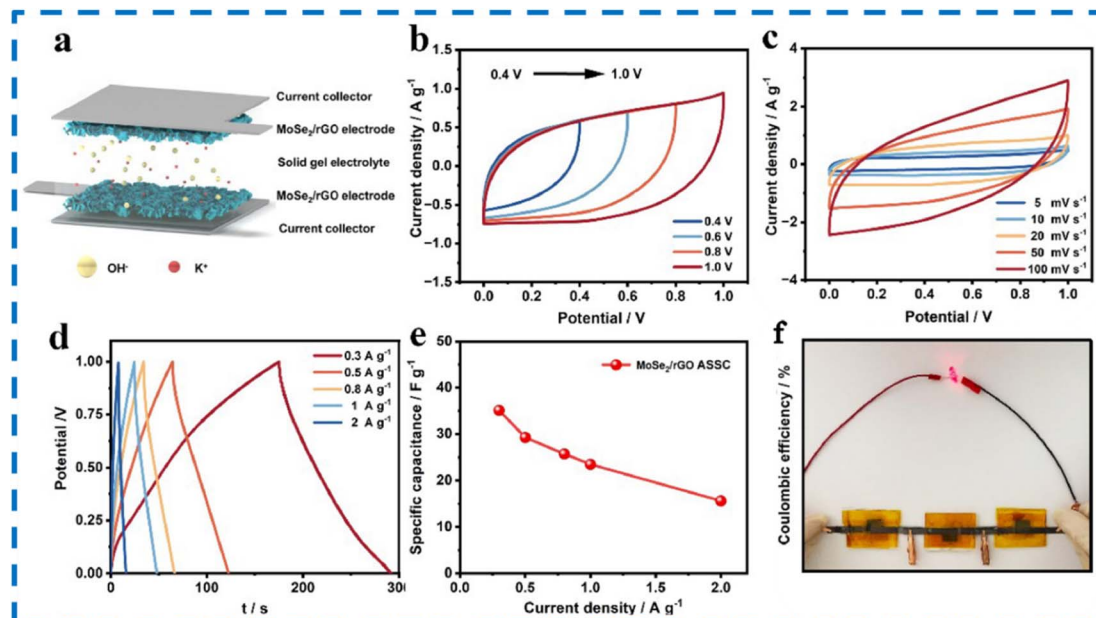
Fig. 17 (a) Schematic of the assembled MoSe 2 /rGO ASSC device (b) CV plots with varying potential windows (c) CV plots at different scanning speeds. (d) GCD plots at different current densities. (e) Specific capacitance evaluated from GCD (f) few serially connected ASSC devices to glow a small LED. This figure has been reproduced from ref. 98 with permission from Elsevier, Copyright 2023.
