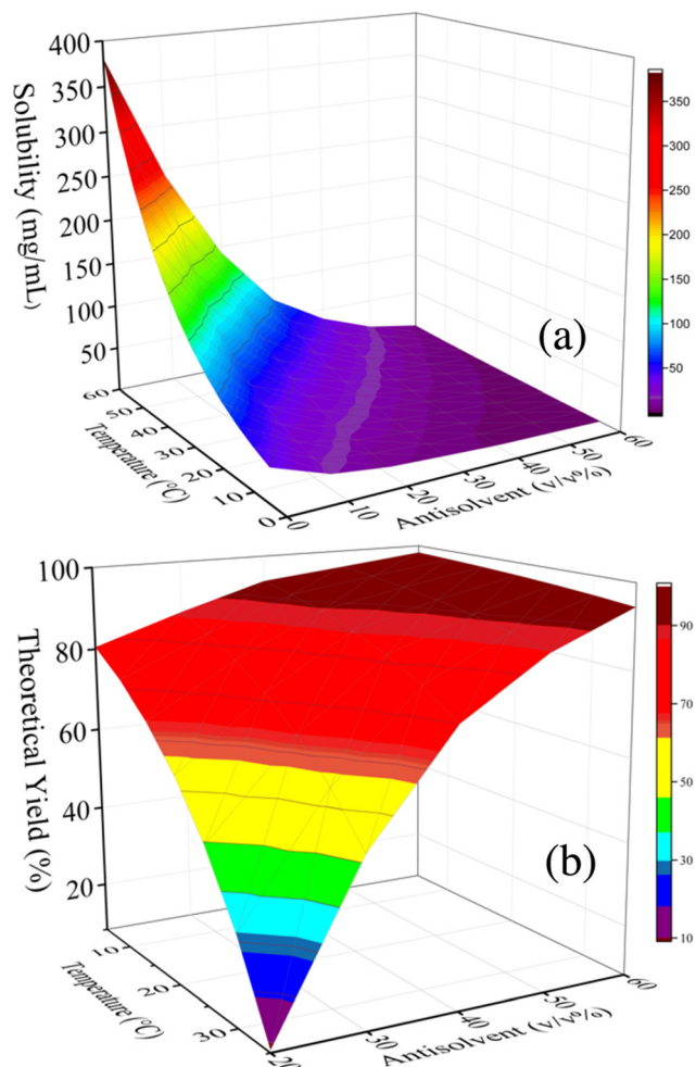
Fig. 3 a. Surface plots for (a) the solubility of commercial modafinil ( 1 ) in the ternary solvent system MEK + formic acid + water [43 : 35 : 22 (v/v)] as a function of temperature and antisolvent (aqueous saturated sodium carbonate) content correlated with exponential equations (Fig. S7 † ) and (b) theoretical yield of 1 in a theoretical crystallization process as a function of temperature and antisolvent content for a feed concentration of 43 mg mL -1 .
