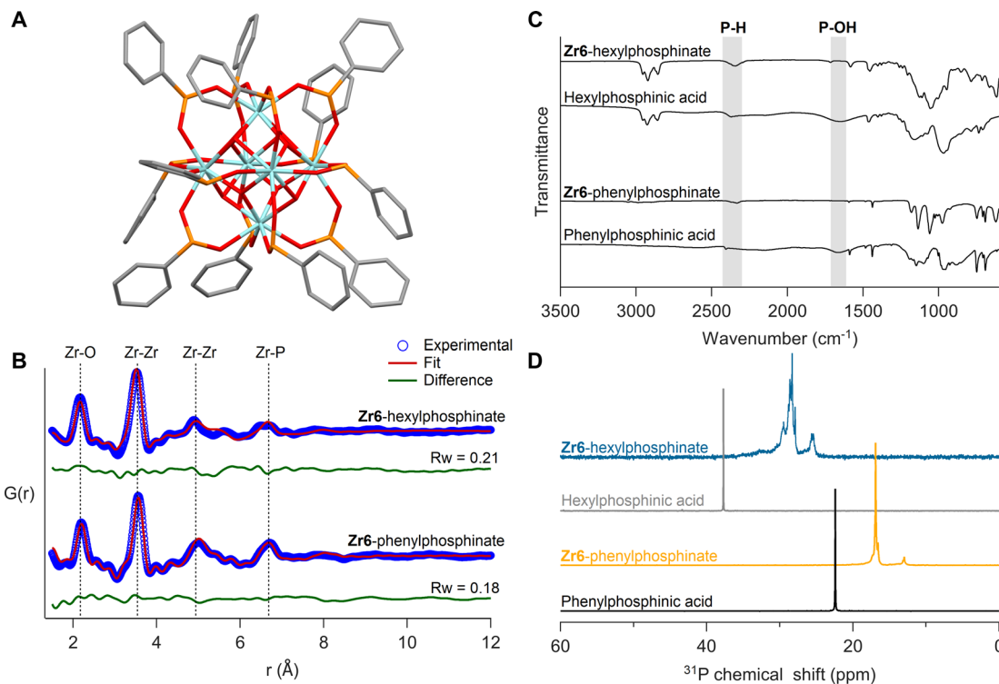
Fig. 6 (A) Crystal structure of Zr 6 -phenylphosphinate cluster – Zr 6 O 8 H 4 (O 2 PHPh) 12 . Cyan atoms represent zirconium and all other atoms follow conventional CPK coloring. The co-crystallized dichloromethane molecules and hydrogen atoms are omitted for clarity. (B) PDF fit for Zr 6 -phenylphosphinate cluster with its crystal structure. PDF fit of Zr 6 -hexylphosphinate cluster with distorted Zr 6 phosphinate cluster is also shown. (C) FTIR spectra of Zr 6 phosphinate clusters. IR spectra of free ligands are also provided for reference. (D) 31 P NMR of purified Zr 6 phosphinate clusters. 31 P NMR of free acids are provided as reference.
