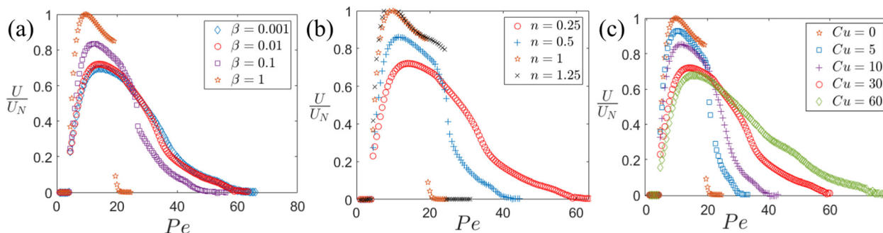
Fig. 7 Variation of normalized axial phoretic velocity of the isotropic colloid with Pe for different values of (a) \beta = (0.001, 0.01, 0.1, 1) for Cu = 30, n = 0.25 , (b) n = (0.25, 0.5, 1, 1.25) for Cu = 30, \beta = 0.01 and (c) Cu = (0, 5, 10, 30, 60) for \beta = 0.01, n = 0.5 . The phoretic axial velocity of the particle in a Newtonian fluid at Pe = 10 ( U_N ) is used for normalization.
