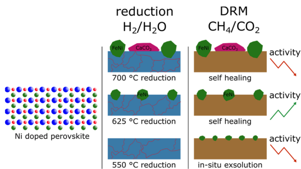
Fig. 9 Summary of the main findings. Differently sized FeNi nanoparticles were created from Ni-doped perovskites by utilising different reduction temperatures. At the highest temperature, additional formation of \text{CaCO}_3 could be observed that, in turn, reduced the catalytic activity. During the reduction, the perovskite started to decompose, but under DRM conditions, the decomposition phases formed a brownmillerite phase again presenting a self-healing factor.
