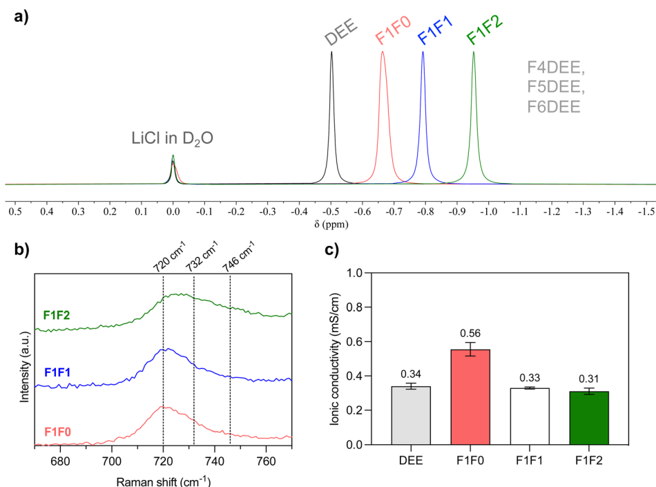
Fig. 2 (a) Overlay of normalized {}^7\text{Li} NMR spectra of electrolyte solutions containing 1.2 mole \text{L}^{-1} of LiFSI salt, and LiCl in \text{D}_2\text{O} was applied as an internal standard. The pale blue region indicates the chemical shift of F4DEE, F5DEE and F6DEE electrolytes in the previous report. (b) Raman spectra of electrolytes in this study showing the solvation conditions of LiFSI salt. (c) Comparison of ionic conductivity in the stainless steel-separator-stainless steel sandwich structure using the Celgard 2325 trilayer separator. Each electrolyte was measured three times (see Table S3†).
