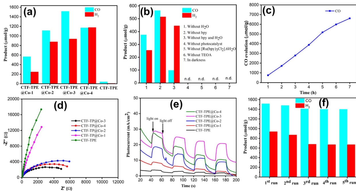
Fig. 6 (a) CO evolution using different Co-loaded CTF- n ( n = 1, 2, 3, 4 ), and a negligible amount of formate is not shown. (b) Reaction conditions for \text{CO}_2 reduction. (c) 7 h long photocatalytic run using CTF-TPE@Co-3. (d) EIS Nyquist plot. (e) Transient photocurrent response of CTF-TPE@Co- n ( n = 1 to 4). (f) Recyclability test of CTF-TPE@Co-3.
