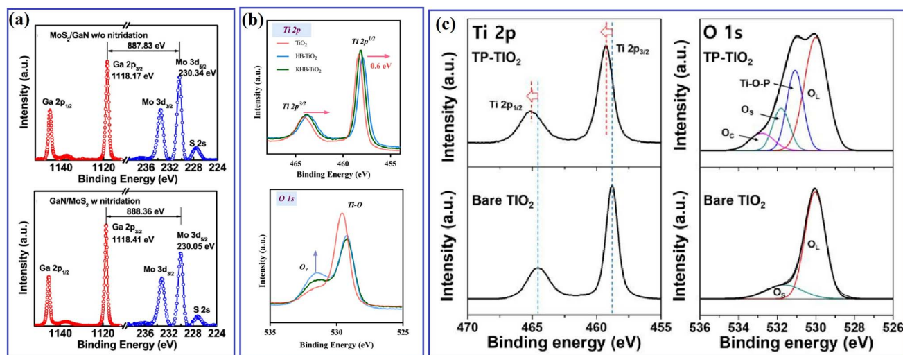
Fig. 11 (a) Ga 2p and Mo 3d core-level spectra obtained from the MoS _2 /GaN interface without and with nitridation treatment. Reproduced with permission from ref. 61. Copyright 2018, the American Chemical Society. (b) Ti 2p and O 1s XPS spectra of TiO _2 , HB-TiO _2 and KHB-TiO _2 . Reproduced with permission from ref. 65. Copyright 2023, Elsevier. (c) Ti 2p and O 1s XPS spectra of bare TiO _2 and TP-TiO _2 . Reproduced with permission from ref. 67. Copyright 2018, MDPI.
