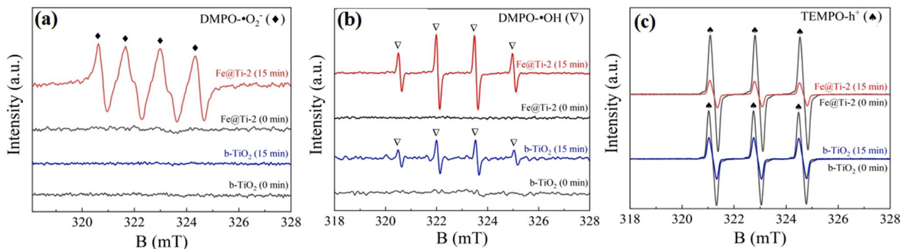
Fig. 10 EPR spectra of Fe@Ti-2 for (a) DMPO- \cdot O _2^- , (b) DMPO- \cdot OH and (c) TEMPO- h^+ . Reproduced with permission from ref. 84. Copyright 2022, Elsevier.
