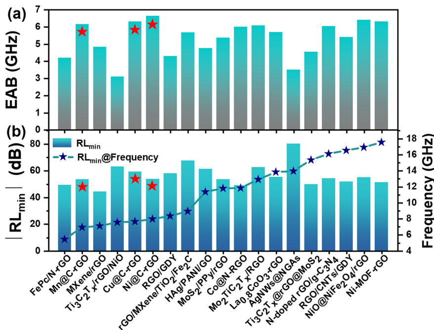
Fig. 4 Comparison of microwave absorption properties: (a) EAB and (b) RL_{\min} versus f of reported graphene-based absorbers.
