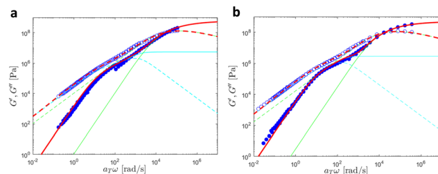
Fig. 15 Linear viscoelastic mastercurves of (a) PMA at T_{ref} = 30 °C and (b) PBA at T_{ref} = -30 °C. Red lines correspond to the model predictions obtained with the values shown in Tables 1 and 2. The contributions from the KWW model (in green) and the Rouse model (in cyan) are also presented.
