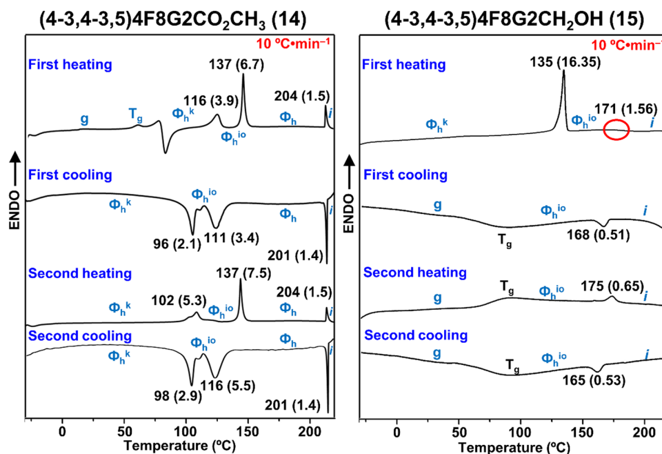
Fig. 1 DSC traces collected for (4-3,4-3,5)4F8G2CO 2 CH 3 ( 14 ) and (4-3,4-3,5)4F8G2CH 2 OH ( 15 ) at heating and cooling rate of 10 °C min -1 . Phases determined by XRD, transition temperatures (in °C), and associated enthalpy changes (in between parentheses in kcal mol -1 ) are indicated. \Phi_h^k , crystalline columnar hexagonal phase; \Phi_h^{\text{io}} , columnar hexagonal phase with intracolumnar order; \Phi_h , liquid crystalline columnar hexagonal phase; i , isotropic phase; g , glassy phase.
