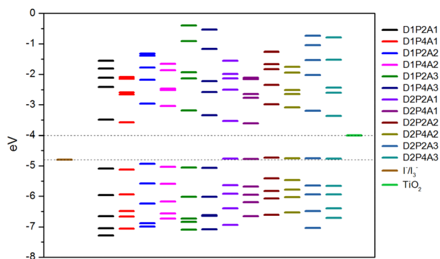
Fig. 1 Selected MOs energy levels for the designed dyes at the B3LYP/6-311+G(2d,p)/SMD level together with TiO 2 CB and \text{I}^-/\text{I}_3^- redox potential.
