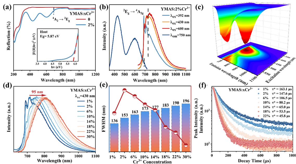
Fig. 2 (a) UV-vis-NIR DR spectra of YMAS: x\text{Cr}^{3+} ( x = 0, 2\% ). The illustration is the optical band gap of the YMAS host. (b) PL and PLE spectra of YMAS: 2\%\text{Cr}^{3+} . (c) The PL mapping spectrum of YMAS: 2\%\text{Cr}^{3+} . (d) Normalized PL spectra of YMAS: x\text{Cr}^{3+} ( x = 1\text{--}30\% ). (e) Luminescence peak intensity and FWHM of YMAS: x\text{Cr}^{3+} ( x = 1\text{--}30\% ). (f) Fluorescence decay curves of YMAS: x\text{Cr}^{3+} ( x = 1\text{--}22\% ) at the optimal monitoring wavelength (715–810 nm).
