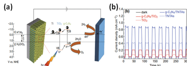
Fig. 6 (a) A schematic depiction of the charge transfer mechanism of the g-C 3 N 4 /TNTA heterojunction electrode. (b) Time-dependent photocurrent density under intermittent light irradiation. Reprinted from ref. 184 with permission.
