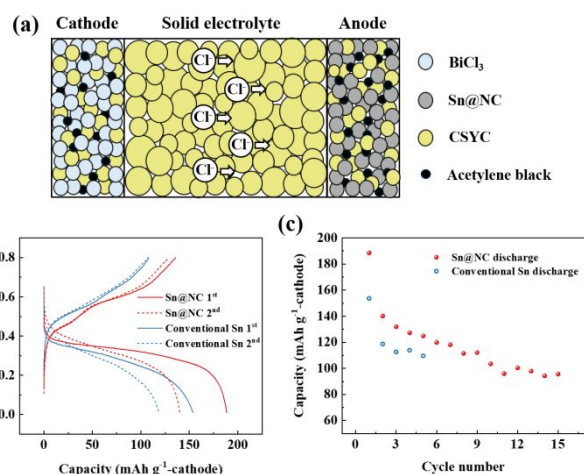
Fig. 4 (a) Schematic diagram of the all-solid-state Cl-ion battery; (b) charge–discharge profiles; and (c) cycling performance of the Sn@NC/CSYC/ BiCl_3 and conventional Sn/CSYC/ BiCl_3 cells.
