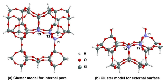
Fig. 2 Cluster models for (a) the internal pore, and (b) the external surface binding sites for REE nitrates in MCM-22 highlighting the T1, T2 and T3 sites.
