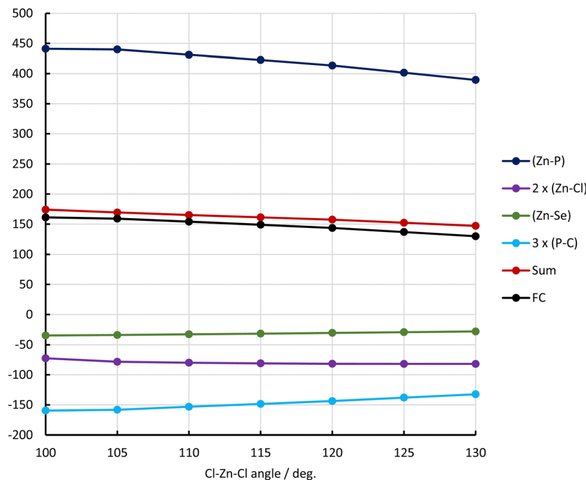
Fig. 5 Dependence of LMO contributions to ^1\text{J}(\text{Zn-P})/\text{Hz} on the Cl–Zn–Cl angle in \text{LZnCl}_2 . Pipek–Mezey localization.
