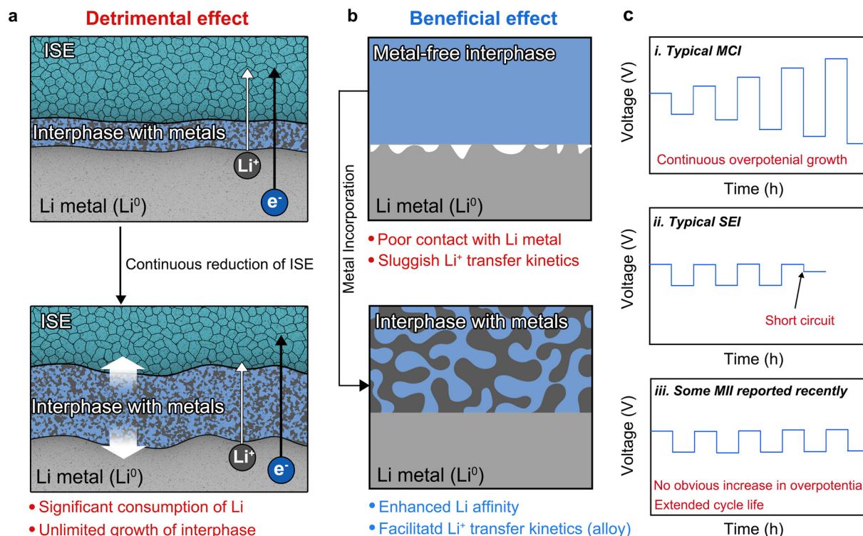
Fig. 1 (a) The schematic diagram of the detrimental effect. (b) The schematic diagram of the beneficial effect. (c) The schematic comparison between Li symmetric cells employing a typical mixed-conducting interphase, a typical solid electrolyte interphase and some metal-incorporated interphases reported recently during galvanostatic discharging/charging tests.
