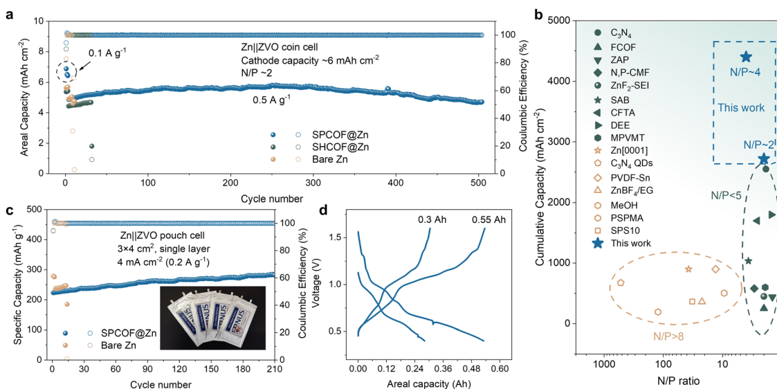
Fig. 7 The performance of Zn metal full cell enabled by SPCOF layer. (a) Cycling performance of Zn||ZVO batteries with different anodes in a 2 \text{ M ZnSO}_4 electrolyte at a low N/P ratio of ~2. The Zn thickness is 20 \mu\text{m} , corresponding to a capacity of \sim 11.7 \text{ mA h cm}^{-2} , with a cathode capacity of \sim 6 \text{ mA h cm}^{-2} . (b) Comparison of N/P ratio and cumulative capacity in this work with prior studies. (c) Cycling performance of 3 \times 4 \text{ cm}^2 Zn||ZVO pouch cells. Inset is optical image of as prepared Zn||ZVO pouch cell. (d) Galvanostatic charge–discharge profiles of 0.3 \text{ A h} and 0.55 \text{ A h} Zn||ZVO pouch cells.
