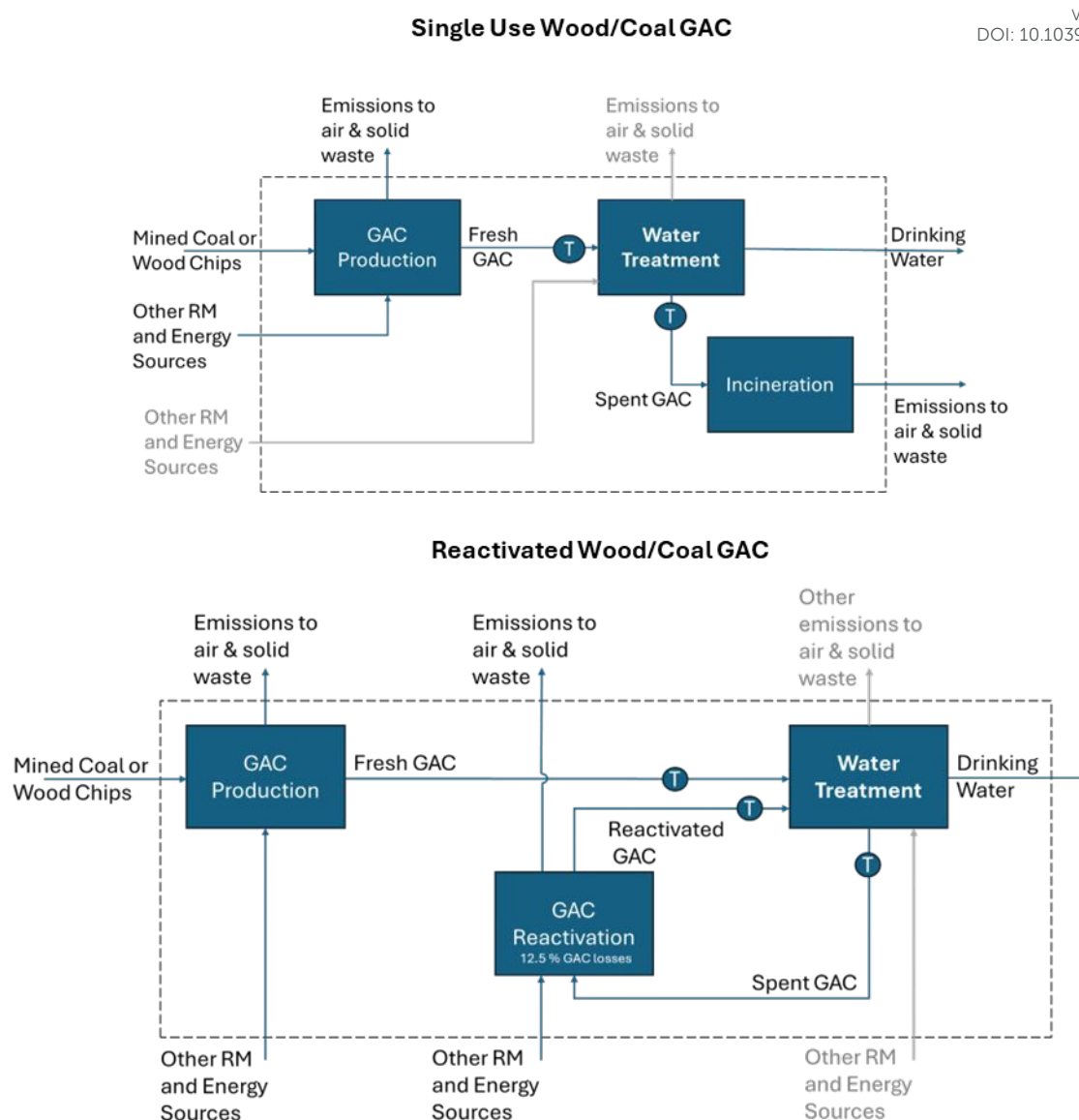
Figure 2: System boundaries considered for single-use and reactivated GAC. Note that as fresh GAC is needed even when using GAC reactivation (to make up for 12.5% losses in each reactivation cycle), the GAC production process is also included within the reactivated GAC system boundaries. Grey in- and out-flows indicate flows in the water treatment process that would not change with updated quality targets and are therefore excluded from the analysis. A circled T indicates transport. RM: Raw materials.
