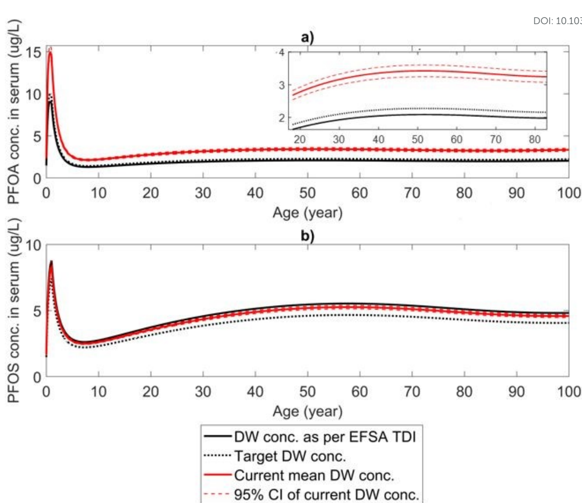
Figure 4: a) PFOA and b) PFOS serum concentrations over someone's lifetime, when drinking water is treated to the EFSA-recommended concentration values, versus when drinking water is kept at the current concentrations, modelled using the EFSA PBPK method. The inserts show the concentrations after age 18. Note that the PFOS concentration is in fact a summed concentration of PFOS and PFHxS. The legend applies to both subplots. DW = drinking water; EFSA = European Food Safety Authority; TDI = tolerable daily intake; CI = confidence interval.
