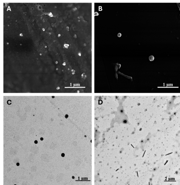
Fig. 3 SEM (A and B) and TEM (C and D) representative micrographs of N13 (A and C) and N11 (B and D) samples.
