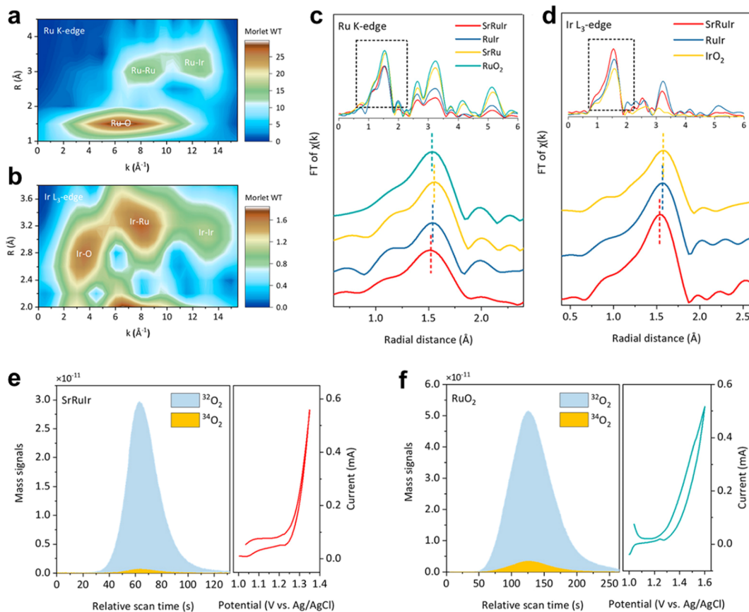
Fig. 18 Structure characterization and OER mechanism analysis of SrRuIr oxide electrocatalyst. (a) and (b) Ru K-edge and Ir L_{3} -edge WT-EXAFS spectra of SrRuIr. (c) and (d) Ru K-edge FT-EXAFS spectra (and Ir L_{3} -edge FT-EXAFS spectra of different samples, respectively). (e) and (f) DEMS signals of ^{32}\text{O}_2 ( ^{16}\text{O}^{16}\text{O} ) and ^{34}\text{O}_2 ( ^{16}\text{O}^{18}\text{O} ) from the reaction products for ^{18}\text{O} -labeled SrRuIr and \text{RuO}_2 catalysts in \text{H}_2 ^{18}\text{O} aqueous sulfuric acid electrolyte and corresponding CV cycles. Reprinted with permission from ref. 112 Copyright 2021, American Chemical Society.
