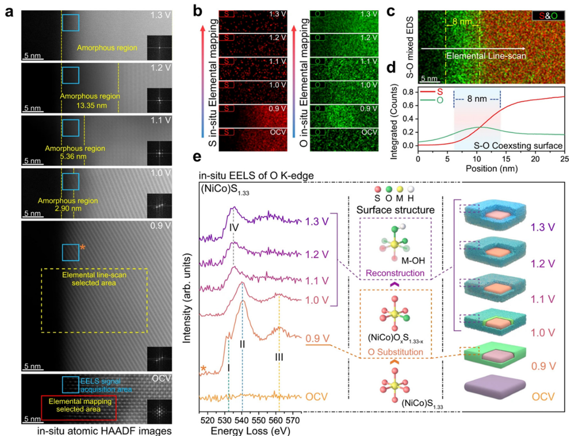
Fig. 14 The exchange of lattice sulphur with oxygen. (a) In situ atomic HAADF images of (NiCo) 1.33 after constantly applying different potentials for 20 s. (b) In situ elemental mapping of S and O under different applied potentials. (c) S–O mixed elemental mapping of (NiCo) 1.33 after constantly applying potentials of 0.9 V for 20 s. (d) The corresponding elemental distribution curve extracted from (c). (e) In situ EELS spectra of O K-edge under different applied potentials. Reprinted with permission from ref. 74 Copyright 2023, Springer Nature.
