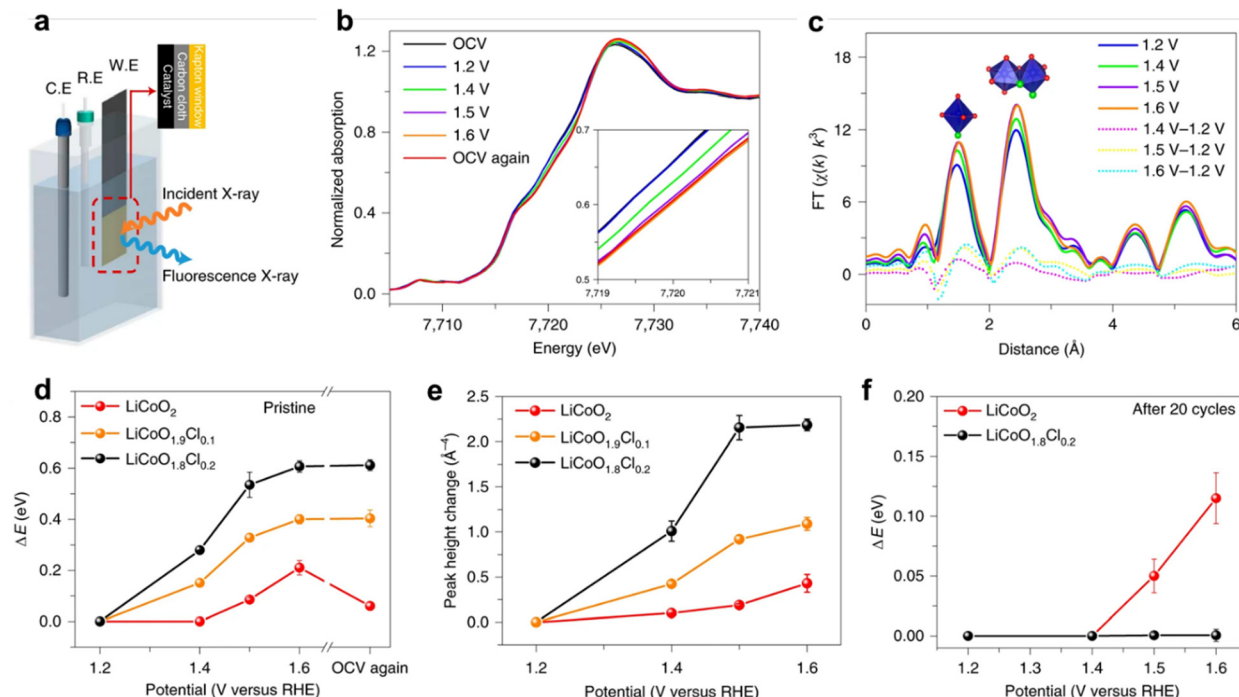
Fig. 8 Operando XAFS test. (a) Experimental set-up scheme. C.E., counter electrode; R.E., reference electrode; W.E., working electrode. (b) and (c) Co K-edge XANES spectra recorded at different potentials for fresh \text{LiCo}_{0.18}\text{Cl}_{0.2} (b) and the corresponding Fourier-transformed k^3 -weighted EXAFS (c). Co K-edge shift (d) and Co–Co coordination peak amplitude change (e) at varied electrochemical potentials for fresh samples. (f) Co K-edge shift for cycled samples (20 times). Reprinted with permission from ref. 35 Copyright 2021, Springer Nature.
