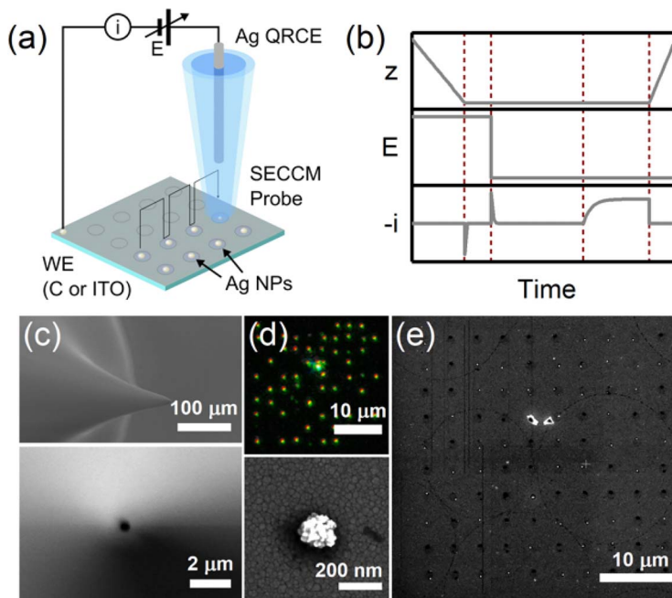
Fig. 1 Applying SECCM to probe electrochemical nucleation and growth. (a) Experimental schematic depicting hopping-mode SECCM measurements. (b) Probe-sample distance, applied potential, and measured current during a single SECCM measurement cycle. (c) SEM images of a typical pipet employed as an SECCM probe. (d) Optical and (e) SEM images of a Ag NP array produced via SECCM on ITO. The bottom panel gives a magnified view of the resulting particle geometry.
