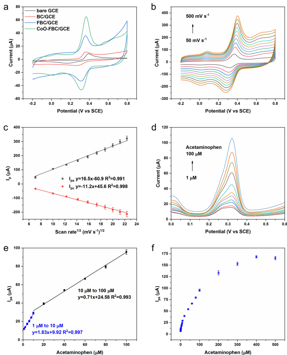
Fig. 5 (a) CV spectra of the bare GCE and biomass derived carbon electrocatalyst modified GCE in APAP solution (500 \mu\text{M} in 0.1 M PBS, scan rate 50 \text{ mV s}^{-1} ); (b) CoO-FBC/GCE CV spectrum in 500 \mu\text{M} APAP in 0.1 M PBS with a changing scan rate; (c) the linear fit of the I_{pa} and I_{pc} current versus the square root of the scan rate in (b); (d) DPV measurement of APAP in 0.1 M PBS with varying concentrations of APAP from 1 \mu\text{M} to 100 \mu\text{M} ; (e) linear fit of DPV I_{pa} current versus the APAP concentrations in (d); (f) DPV I_{pa} current of APAP solution from 1 \mu\text{M} to 500 \mu\text{M} .
