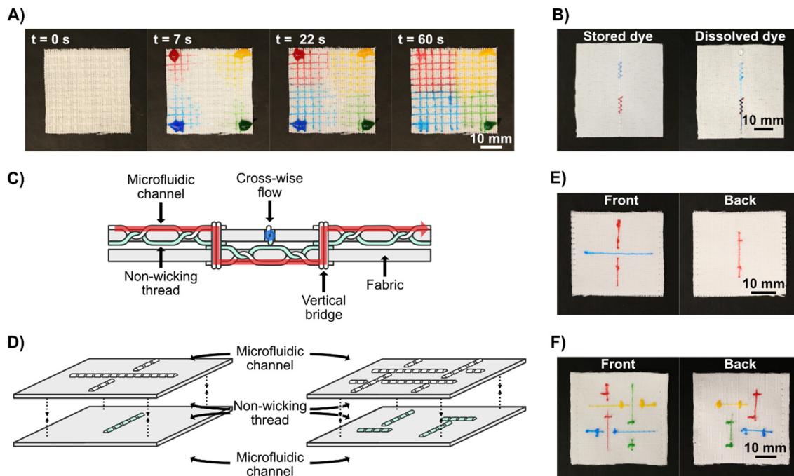
Fig. 3 Advanced microfluidic functions in stitched textile-based microfluidic devices. A) Sequential view of liquid flow through a 4 × 4 cm stitched device with 100 microfluidic channel crossings. B) Demonstration of chemical storage in stitched Coolmax® thread. The zigzag stitches contained dried dye which was rehydrated and transported with the liquid flow after MilliQ water was added to one end of the straight stitch (top of the picture as shown). As the water passes through both storage regions, the colors of the dyes mix. C) Sideview schematic of the 3D stitched microfluidic device. The microfluidic channels of the two layers, aligned through the z-axis, are connected with stitches that pass through both layers vertically. Since there is no fluid path between the perpendicular flows on the top and bottom faces of the device, they do not mix. D) Oblique schematic view of the 3D stitched microfluidic device. Two layers of hydrophobic fabric are stitched with Coolmax® as the spool thread and non-wicking nylon monofilament as the bobbin thread. The faces of the fabrics with the non-wicking thread are stitched together facing each other. E) Photographs of the two faces of a complete 3D stitched textile-based microfluidic device with a single underpass crossing, showing that the flows of the two different dyes (blue and red) were kept separate. F) Photographs of the two faces of a complete 3D stitched textile-based microfluidic device with four intertangled microfluidic channels, with separated liquid flows.
