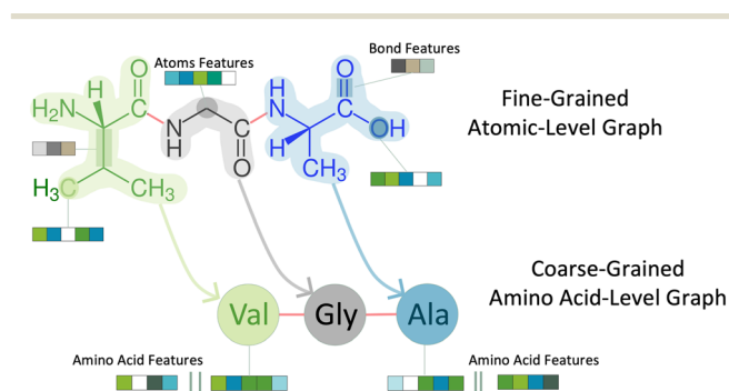
Fig. 1 Construction of atomic-level graph from amino acid sequence.
