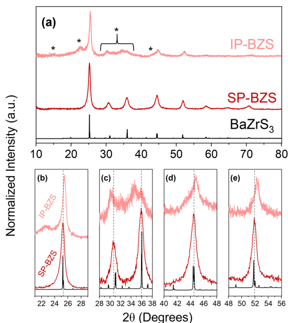
Fig. 1 Structural characterization of synthesized BaZrS 3 nanoparticles via pXRD of both obtained species shown in (a). The peaks labelled with * are the most easily identifiable additional peaks or differences that show in IP-BZS that are not present in SP-BZS. A comparison of the major peak positions between the two BaZrS 3 phases synthesized in this work is shown in (b)–(e). In black is the BaZrS 3 standard (ICSD# 23288), in dark red is SP-BZS, and in pink is IP-BZS. We note that in (c), several differences are present including peak shifts and additional peaks in IP-BZS.
