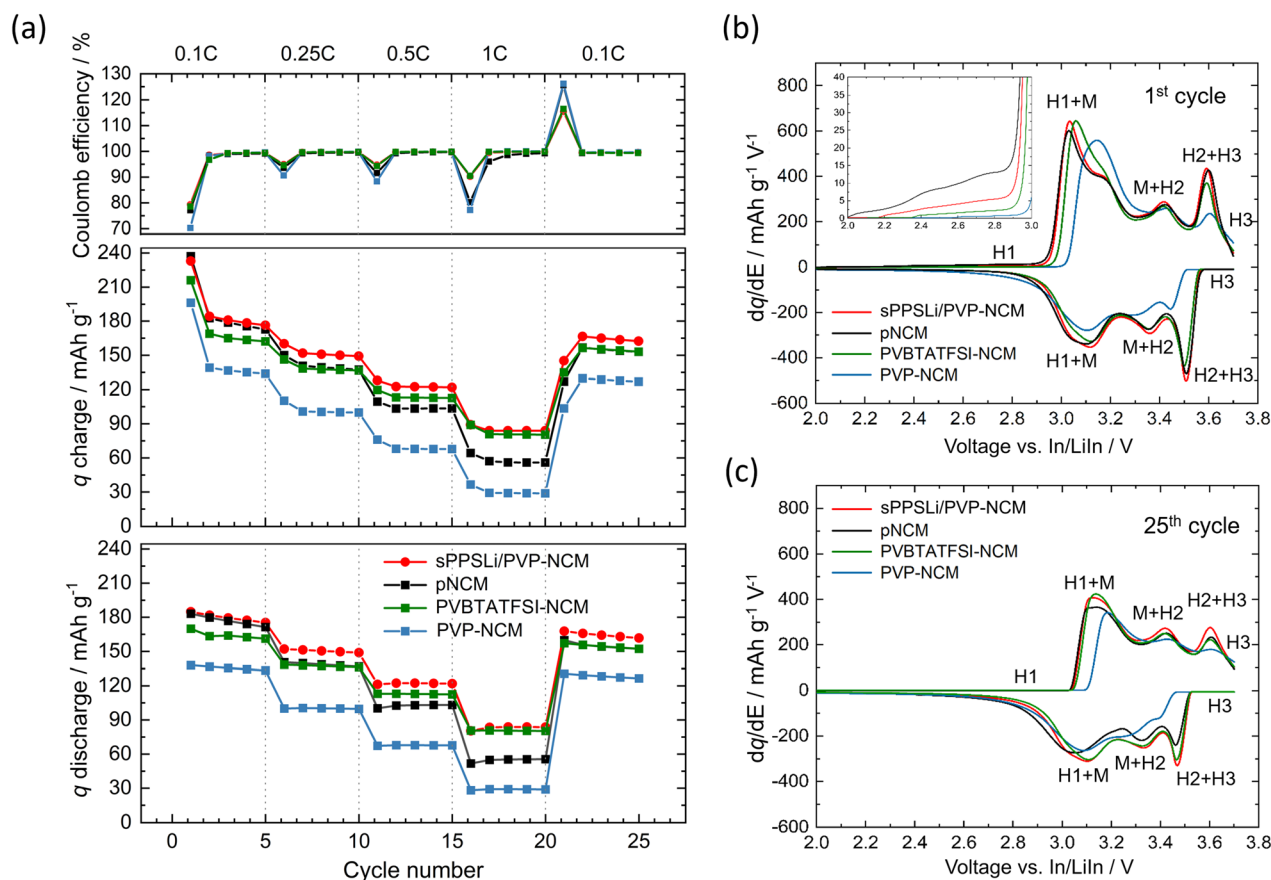
Fig. 3 (a) Specific capacity q and Coulomb efficiency at different C-rates of \text{LiInSEB}^{\text{NCM}} using pNCM, sPSSLi/PVP-NCM, PVP-NCM, or PVBATATFSI-NCM, tested at C-rates of 0.1C to 1C in a pellet-type cell ( \text{LiIn}|\text{Li}_6\text{PS}_5\text{Cl}|\text{Li}_6\text{PS}_5\text{Cl}/\text{VGCF}/\text{NCM} ) with 2.1 \text{ mA h cm}^{-2} nominal area capacity. Differential capacity dq/dE at 0.1C (b) in the 1st cycle and (c) in the 25th cycle. The inset in (b) shows an enlargement from 2–3 V (vs. In/LiIn) of the 1st cycle.
