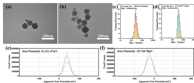
Fig. 4 Characterization of ZIF-8 and ZIF-8@HA. (a) and (b) TEM images, (c) and (d) hydrodynamic size distributions, and (e) and (f) zeta potential distributions of ZIF-8 and ZIF-8@HA.
