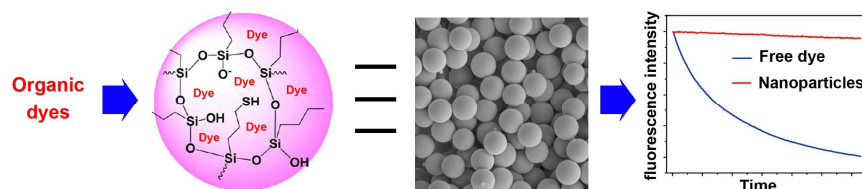
Fig. 2 Schematic diagram of dye-doped nanoparticles, its representative TEM image, and the enhanced stability of doped fluorophores.
