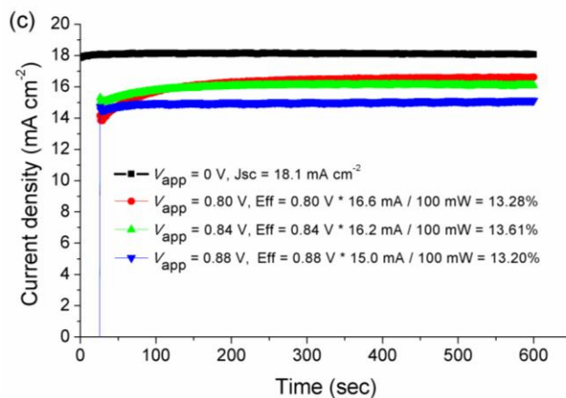
Fig. 7 J-V characteristic curves of “Cell 3” (Table 2) obtained at (a) forward scan direction and different scanning rate, with delaying time ranging from 50, 300 to 500 ms, (b) different scanning directions with delaying time of 50 ms. (c) 10 minutes’ steady photocurrent output at different bias potentials of “Cell 3” under 1 sun illumination.
