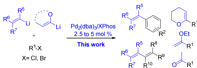
Scheme 1 Palladium catalysed cross-coupling of alkenyllithium reagents
