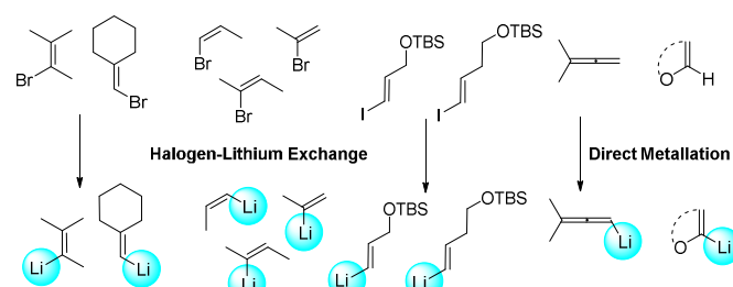
Scheme 2 Synthesis of alkenyllithium reagents.
