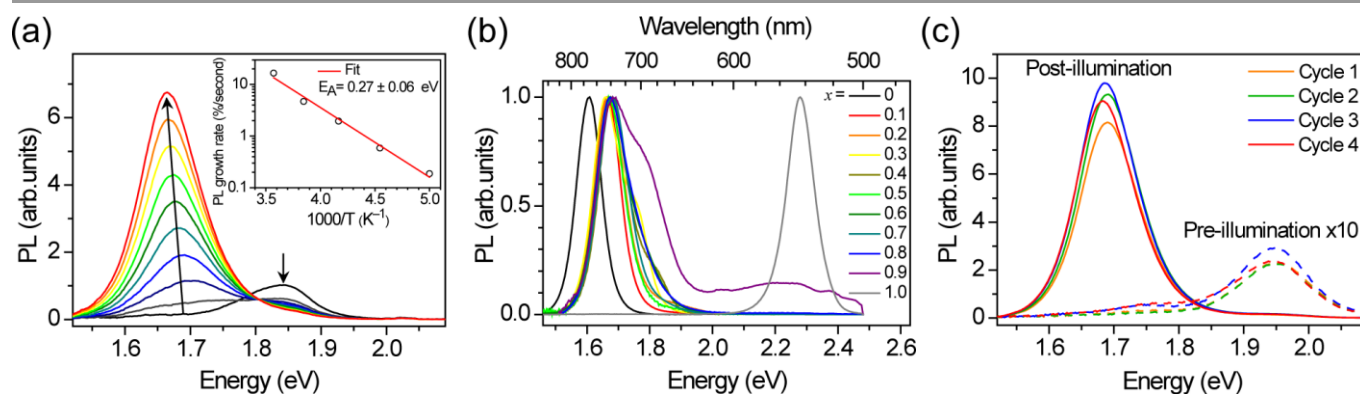
Figure 2. (a) Photoluminescence (PL) spectra of an x = 0.4 thin film over 45 s in 5-s increments under 457 nm, 15 mW/cm 2 light at 300 K. Inset: temperature dependence of initial PL growth rate. (b) Normalized PL spectra of (MA)Pb(Br x I 1-x ) 3 thin films after illuminating for 5–10 minutes with 10–100 mW/cm 2 , 457 nm light. (c) PL spectra of an x = 0.6 thin film after sequential cycles of illumination for 2 minutes (457 nm, 15 mW/cm 2 ) followed by 5 minutes in the dark.
