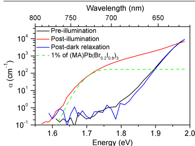
Figure 3. Absorption spectra of an x = 0.6 film before (black) and after (red) white-light soaking for 5 minutes at 100 mW/cm 2 , and after 1 h in the dark (blue). A scaled absorption spectrum of an x = 0.2 film (dashed green) is shown for comparison.
