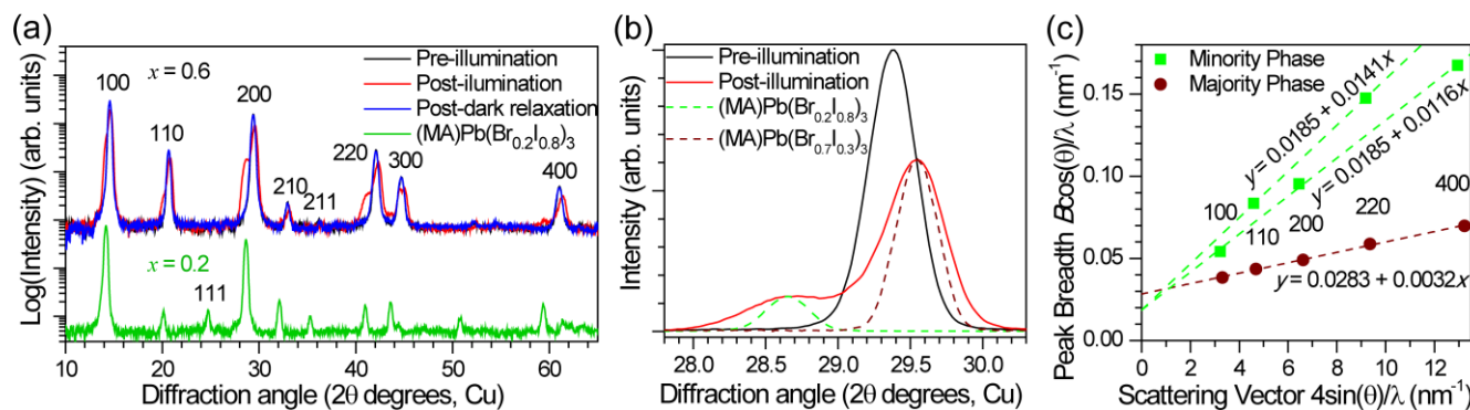
Figure 4. (a) XRD pattern of an x = 0.6 film before (black) and after (red) white-light soaking for 5 minutes at \sim 50 mW/cm 2 , and after 2 h in the dark (blue). The XRD pattern of an x = 0.2 film (green) is offset for comparison. (b) The 200 XRD peak of an x = 0.6 film before (black) and after (red) white-light soaking for 5 minutes at \sim 50 mW/cm 2 . XRD patterns of an x = 0.2 film (dashed green) and an x = 0.7 film (dashed brown) are included for comparison. (c) Williamson-Hall plot of the XRD peak full width at half maximum ( B ) for the minority (green, larger lattice spacing) and majority (brown, smaller lattice spacing) phases observed in (MA)Pb(Br 0.2 I 0.8 ) 3 ( x = 0.6 ) thin films under illumination. \vartheta is the diffraction angle and \lambda = 1.54060 Å (Copper K \alpha 1) is the x-ray wavelength. The points are labeled with their crystallographic indices. Linear regressions to the data are plotted and the equations are listed. The minority phase was fit assuming the same crystallite size in the 100 and 110 directions but different amounts of strain disorder.
