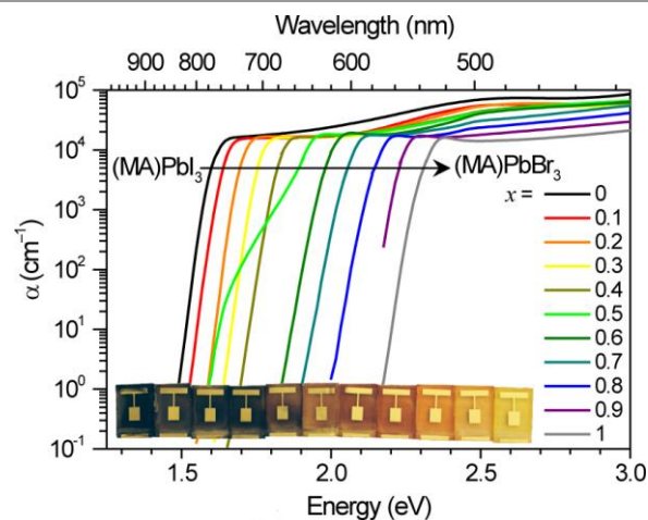
Figure 1. Absorption coefficient of (\text{MA})\text{Pb}(\text{Br}_x\text{I}_{1-x})_3 measured by diffuse spectral reflection and transmission measurements on thin films and photocurrent spectroscopy of solar cells. Inset: photograph of (\text{MA})\text{Pb}(\text{Br}_x\text{I}_{1-x})_3 photovoltaic devices from x = 0 to x = 1 (left to right).
