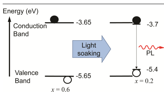
Figure 5. Schematic of the proposed mechanism for photo-induced trap formation through halide segregation. Photogenerated holes or excitons may stabilize the formation of iodide-enriched domains which then dominate the photoluminescence. The valence band (VB) and conduction band (CB) energies with respect to vacuum were estimated by interpolation of published values obtained from ultraviolet photoemission spectroscopy (UPS) and inverse photoemission spectroscopy (IPES) for the endpoint stoichiometries. 35
