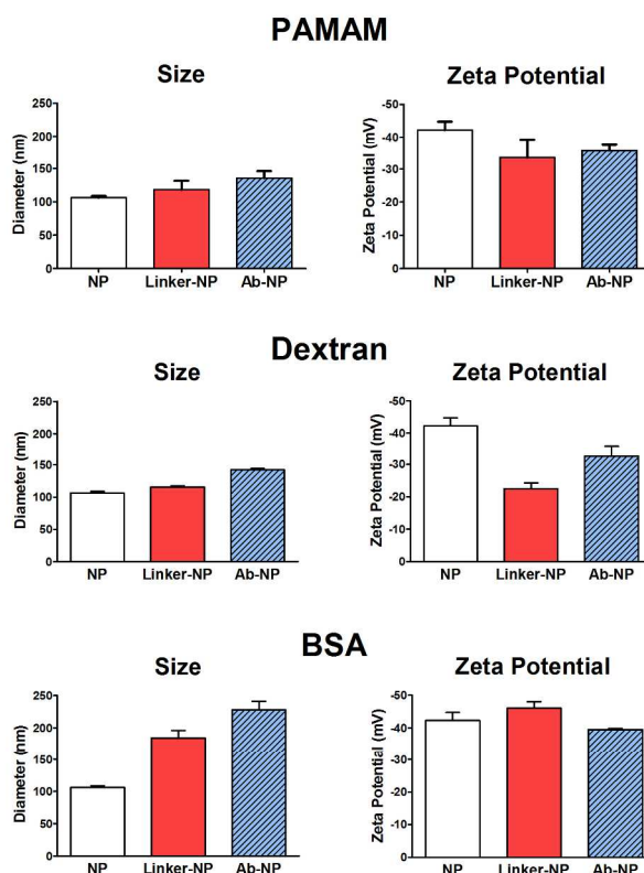
Figure 3. DLS data showing the size and zeta potential evolution of anti-IgG coated NPs prepared using different multivalent linkers. The addition of linker molecules and antibodies to the NP surface induced an increase in particle size. PAMAM and dextran attachment induced NP stability and particle size increases upon linker and antibody attachment were seen. Zeta potential analysis of the NPs showed that PAMAM retained a high negative charge on the NP surface, whilst uncharged dextran produced a more ‘neutral’ colloid. The attachment of BSA led to undesirable ‘growth’ in particle size, attributed initially to the use of glutaraldehyde.
