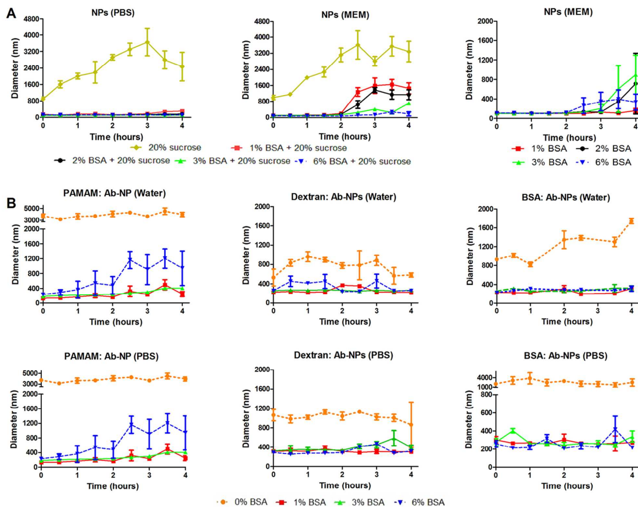
Figure 5 Nanoparticles were freeze-dried from solutions containing various cryoprotectants (described in legends) and redispersed in DI water, PBS or MEM. Redispersion was performed by adding the appropriate medium to the solid form NPs and shaking the dried samples (by hand) back into solution (A) Unmodified NPs were freeze-dried in different concentrations of BSA (right) or BSA solutions containing 20% sucrose (left and centre). The solid form of unmodified NPs was reconstituted in PBS and MEM; (B) With BSA clearly demonstrating a stabilising effect during freeze drying, Ab-NPs prepared with different linkers were redispersed in water and PBS after being freeze-dried in a 0% (i.e. only DI water), 1%, 3% or 6% BSA solution. Following redispersion, the evolution of particle size over time was monitored by DLS.
