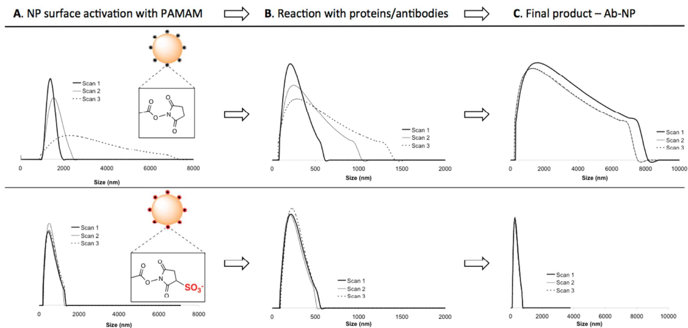
Figure 2 Progress of protein (BSA) conjugation reactions with NPs monitored by dynamic light scattering (DLS). The evolution of the size was measured at different time intervals upon mixing the reagents. In the Step 1, (A) the NPs were reacted with PAMAM dendrimers activated with either EDC-NHS (top) or EDC-Sulfo-NHS (bottom). When bound to the NP surface, the negatively charged, EDC/sulfo-NHS activated dendrimer supported NP stability in solution (unlike EDC/NHS activated PAMAM). Measured time intervals: Scan 1 – 0 min, Scan 2 – 15 min and Scan 3 – 30 min; Step 2; (B) corresponds to the reaction of activated NPs with a Cy5-labeled BSA performed in MES 0.1M pH4.2. Measured time intervals: Scan 1 – 0 min, Scan 2 – 60 min and Scan 3 – 120 min; and (C) Size distributions of the final Ab-NPs following the removal of non-covalently bound protein (measured in triplicate). The use of EDC/sulfo-NHS activated dendrimer resulted in a narrow protein-coated NP size distribution.
