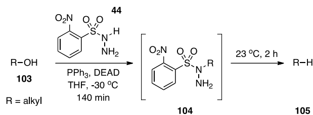
Scheme 37. Deoxygenation of alcohols to alkanes using o -nitrobenzenesulfonylhydrazine 44 .
