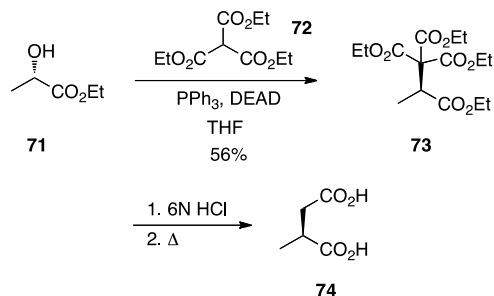
Scheme 22. Carbon-carbon bond formation in the Mitsunobu reaction with the triply-activated methane of triethyl methanetricarboxylate ( 72 ).
