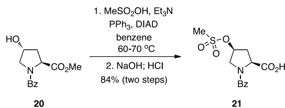
Scheme 7. Synthesis of sulfonate esters employing sulfonic acids as the pronucleophile.
