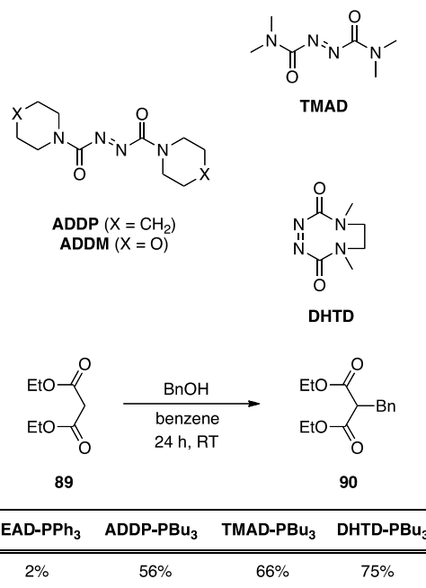
Scheme 29. Comparison of the efficiencies of Mitsunobu co-reagents in the C -alkylation of diethyl malonate.
