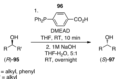
Scheme 33. Built-in phosphine: inversion of a secondary alcohol with a carboxylic acid that also carries the requisite triarylphosphine functionality.
