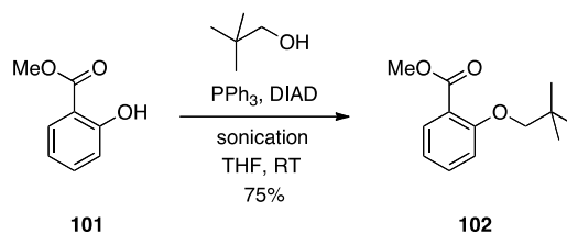
Scheme 36. Sonication assists in difficult Mitsunobu etherifications.
