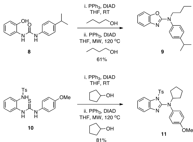
Scheme 4. 2-Ureidophenols and 2-ureidoanilines undergo intramolecular Mitsunobu reactions to deliver N 2 -substituted benzoxazoles and benzimidazoles, respectively.
