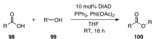
Scheme 34. Towards an organocatalytic Mitsunobu reaction. Note the sub-stoichiometric use of DIAD.
