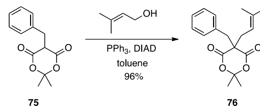
Scheme 23. Alkylation of C^5 -mono-substituted Meldrum's acids.
