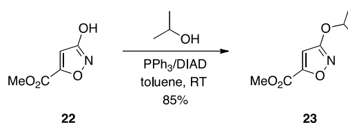
Scheme 8. Regioselective O -alkylation of 3-hydroxyisoxazoles under Mitsunobu control.
