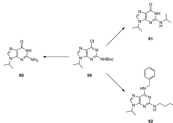
Scheme 18. The versatility of N^9 -substituted- N^2 -Boc-2-amino-6-chloropurine.
