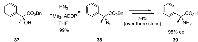
Scheme 12. Synthesis of an \alpha,\alpha -disubstituted amino acid from tertiary \alpha -hydroxy esters.
