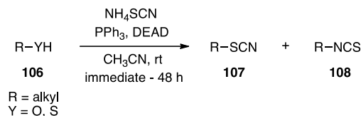
Scheme 38. Synthesis of thiocyanates and isothiocyanates with the thiocyanate anion as the nucleophile.
