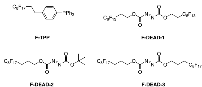
Scheme 35. Fluorous Mitsunobu reagents to facilitate purification of the reaction mixture.
